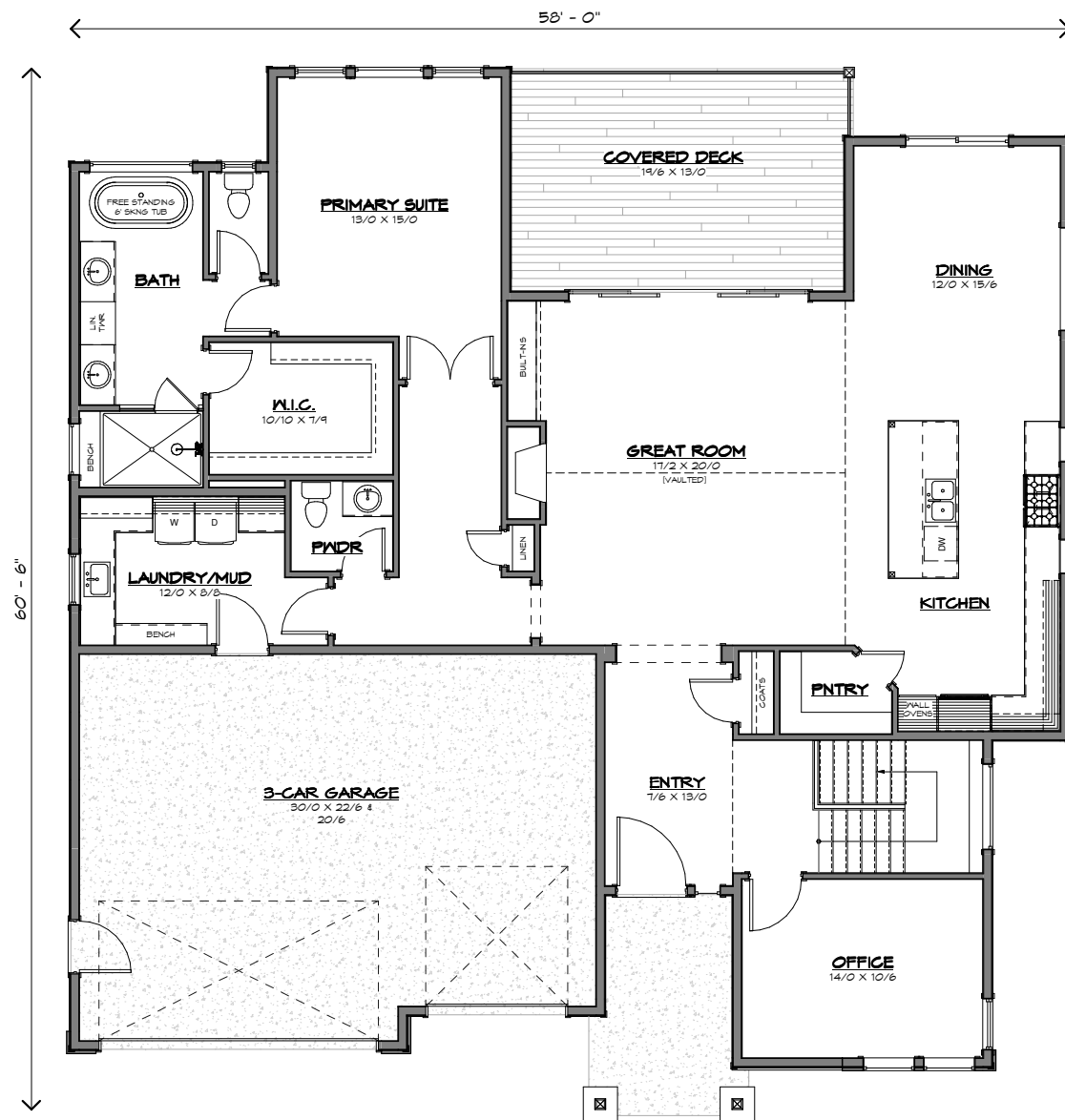
MAIN FLOOR PLAN - 2019 SF
