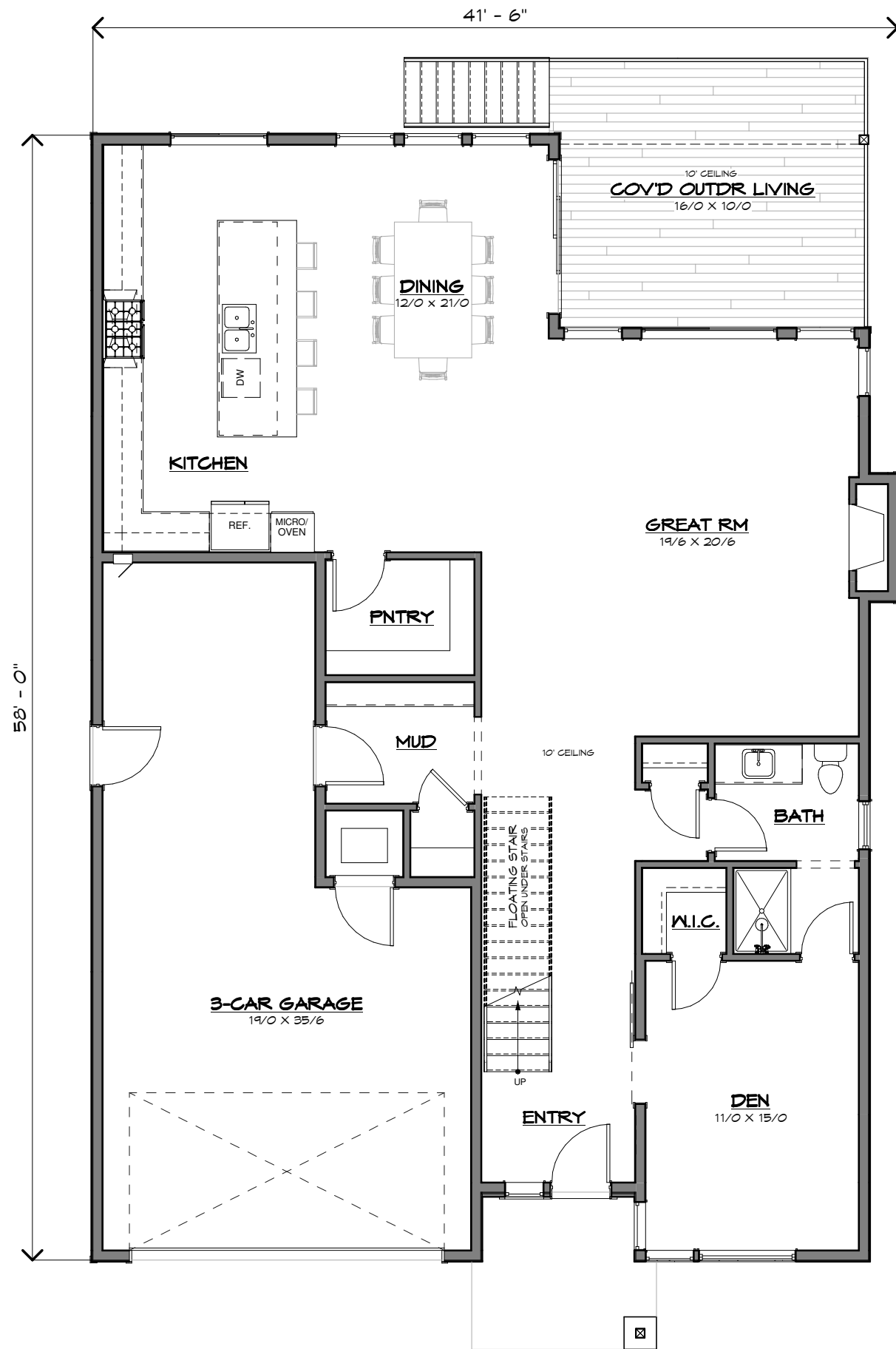
Main Floor Plan - (1571 SF.) 1/4" = 1'-0"
