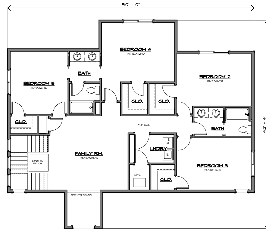
Upper Floor Plan - (1447 SF.) 1/4" = 1'-0"
