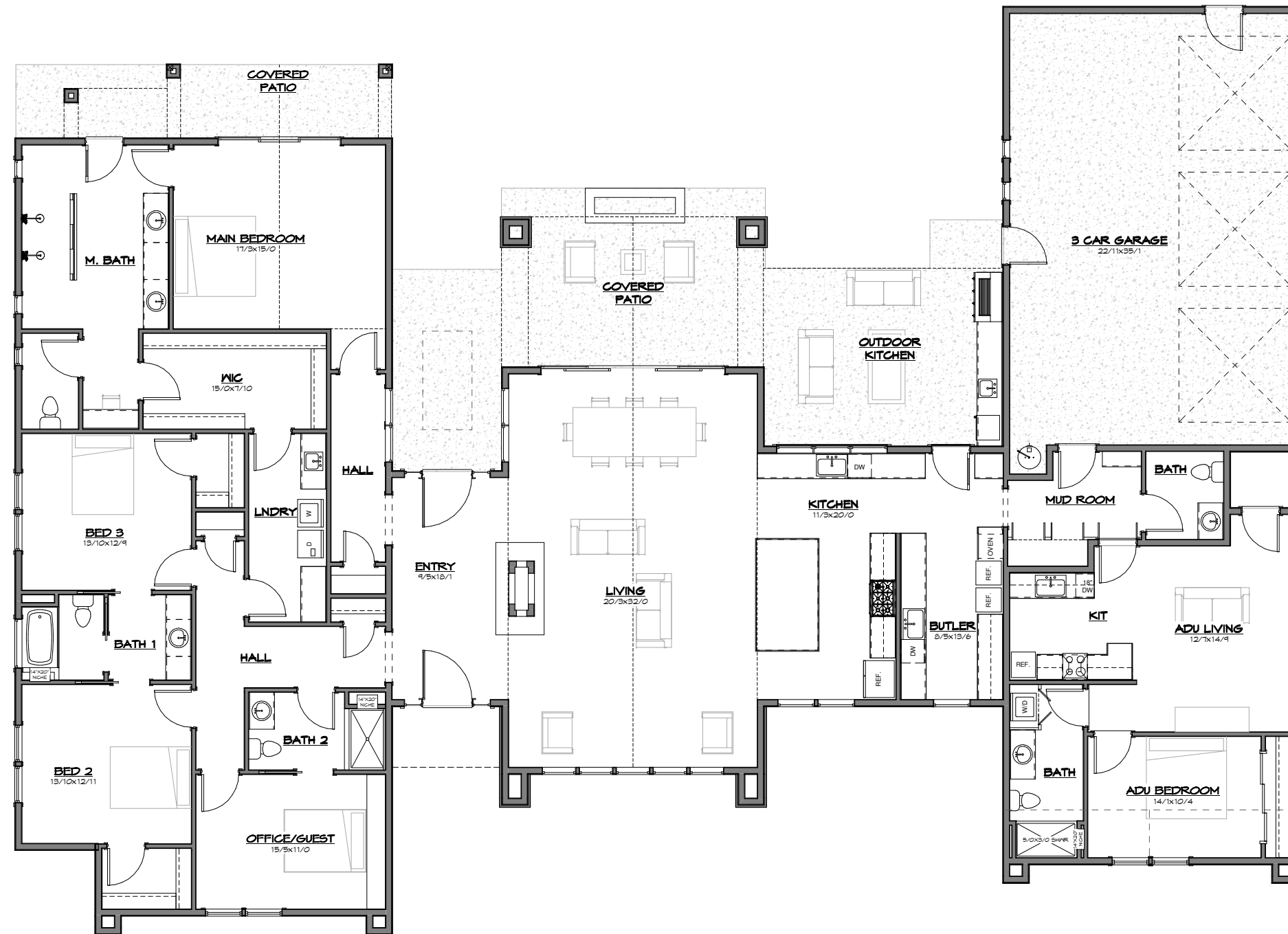
Main Floor Plan - 3,326 SF
